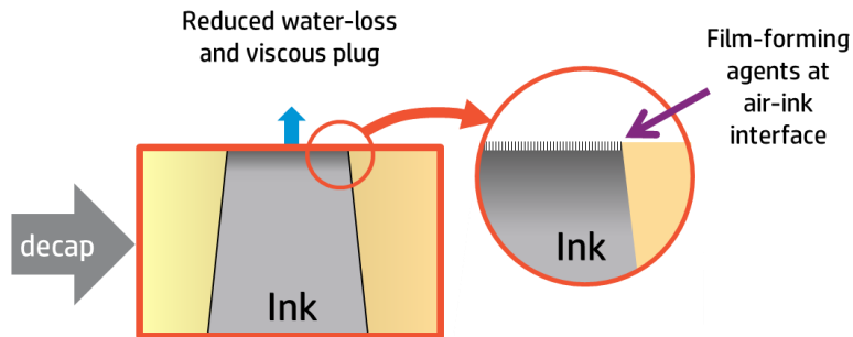
Figure 2. HP PageWide XL Pigment Inks: film-forming functionality
