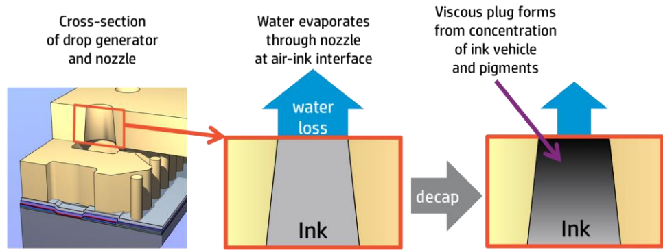
Figure 1. Effects during extended decap time: conventional pigment inks
