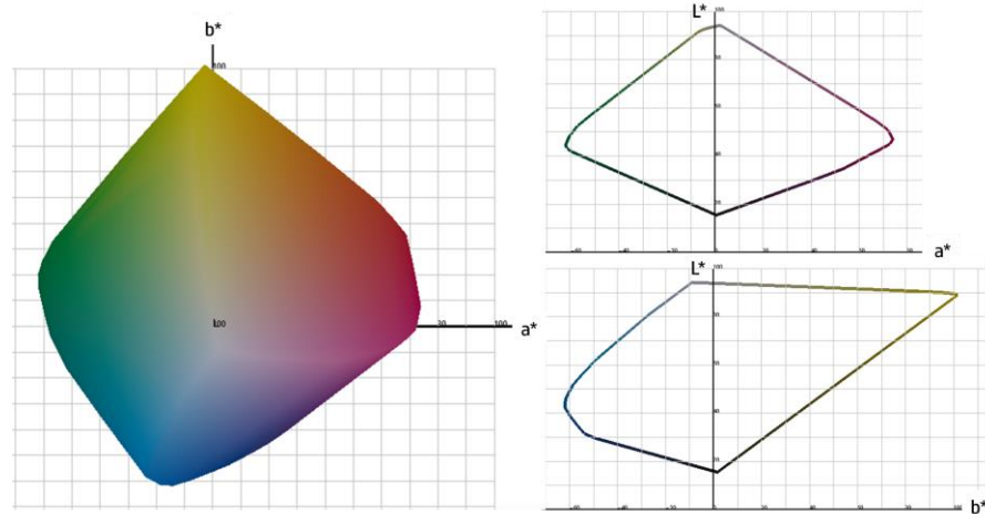
Figure 3. Color gamut of HP PageWide XL Pigment Inks on HP Heavyweight Coated Paper
